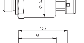
Metri Pack Series 150 P2S
