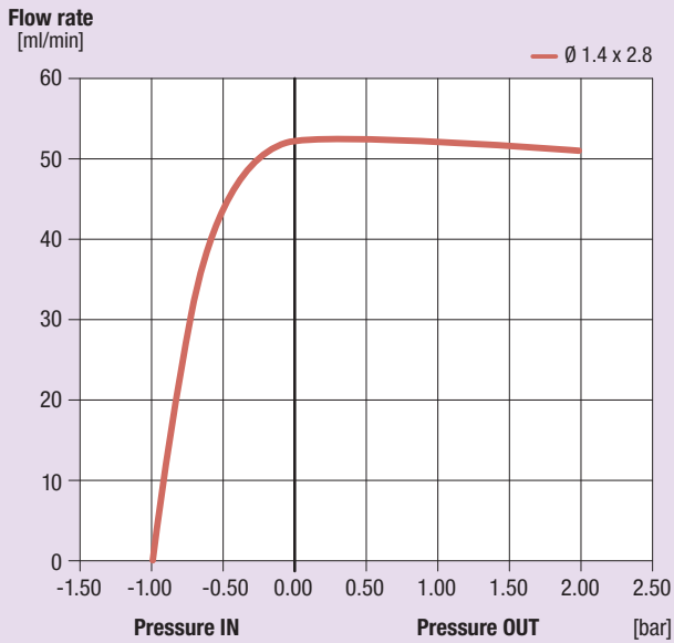
TP16 @ 24 V
