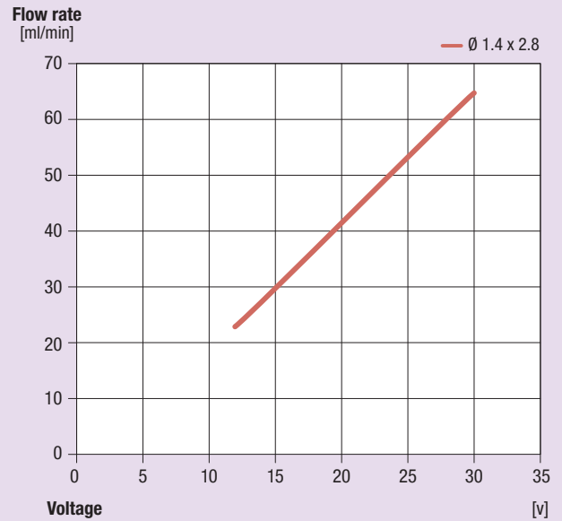
TP16 @ 0 bar
